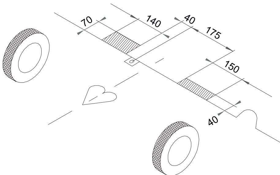
DETAIL 3
